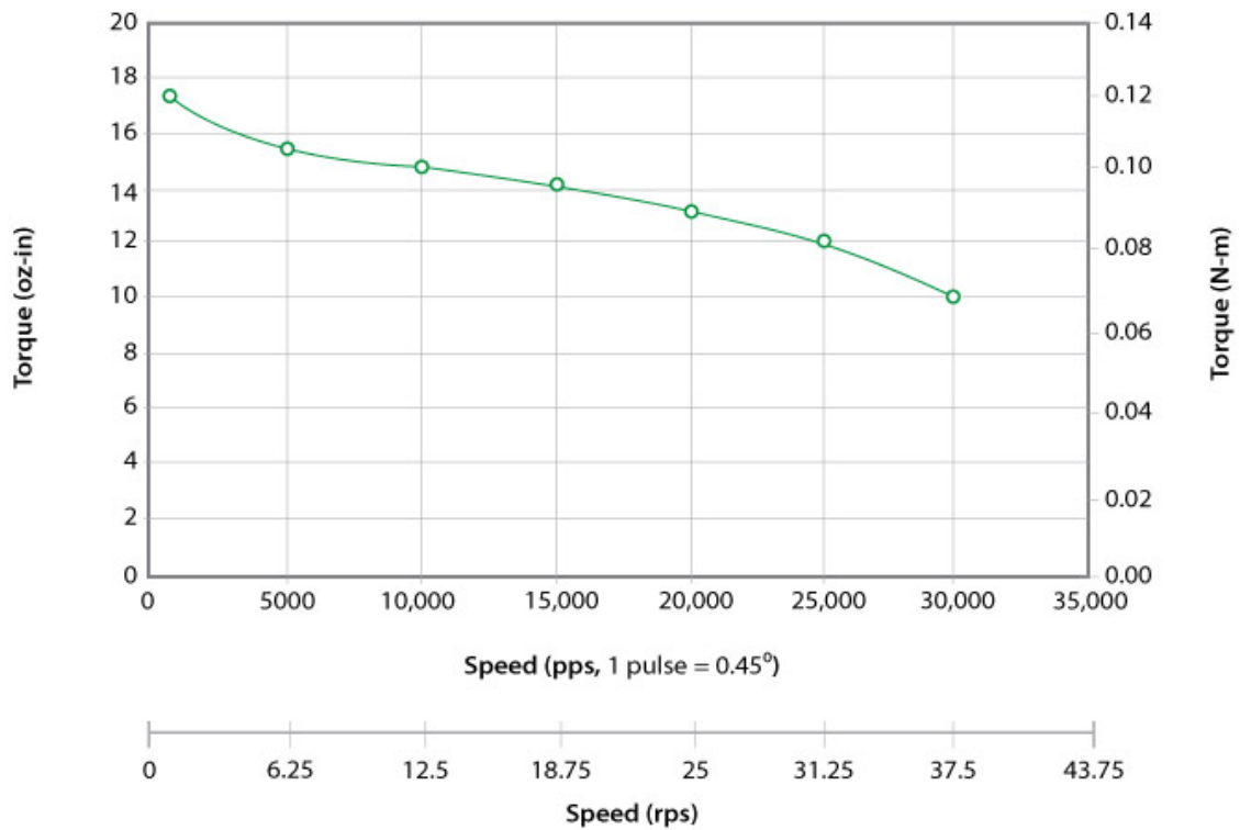
417-15-08 24VDC, 2.0 Amps/Phase, Bipolar, 1/2 Stepping
